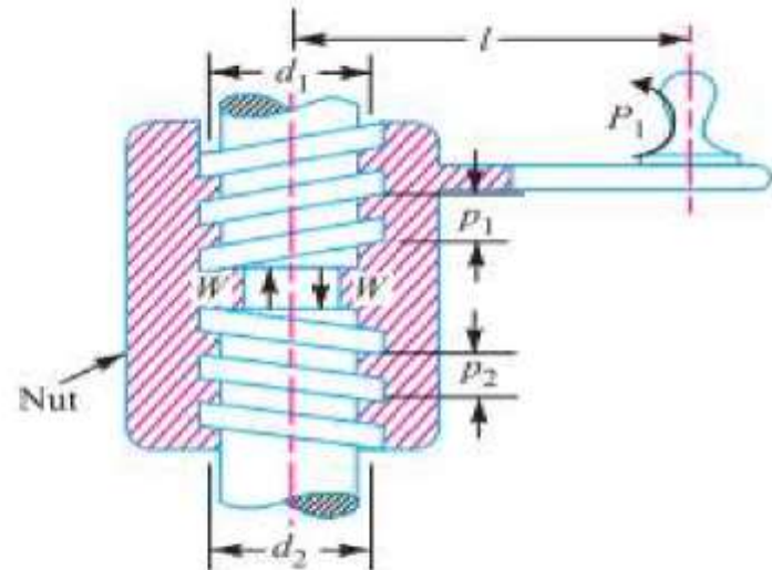
(b) Threads wound on the different cylinders.
