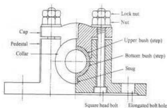
Fig 1.3: Pedestal Bearing
