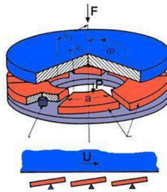
Fig 1.6(a): Fixed-incline-pads thrust bearing Fig 1.6(b): Pivoted-pads thrust bearing
