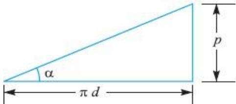
(a) Development of a screw.
