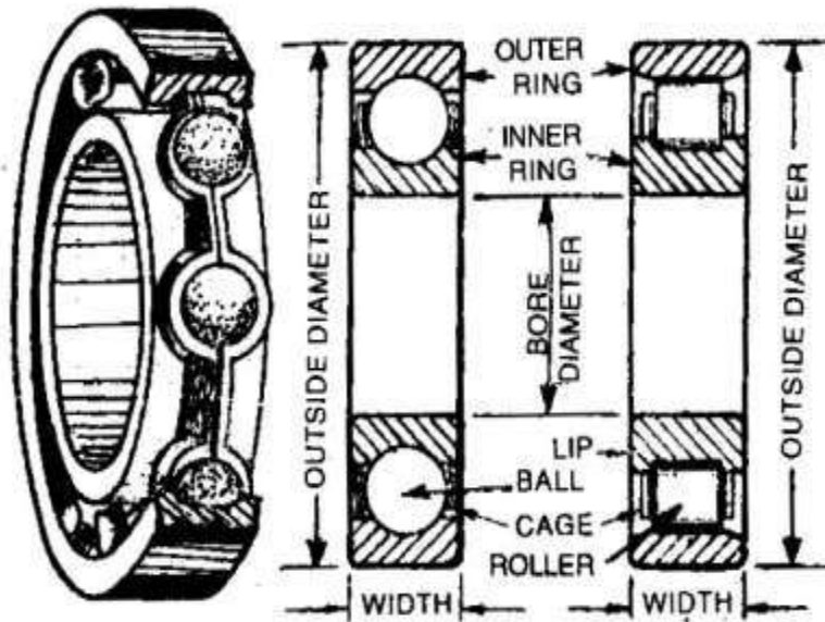
(a) Ball bearing
