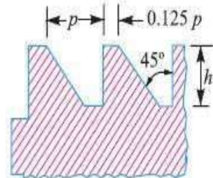
(c) Buttress thread.
